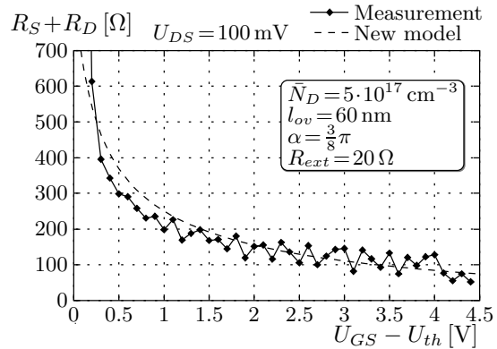
Figure 6: Source and drain resistor measured at MOSFETs with gate lengths between 0.7 and 3 \mu m and 10 \mu m gate width [5]
